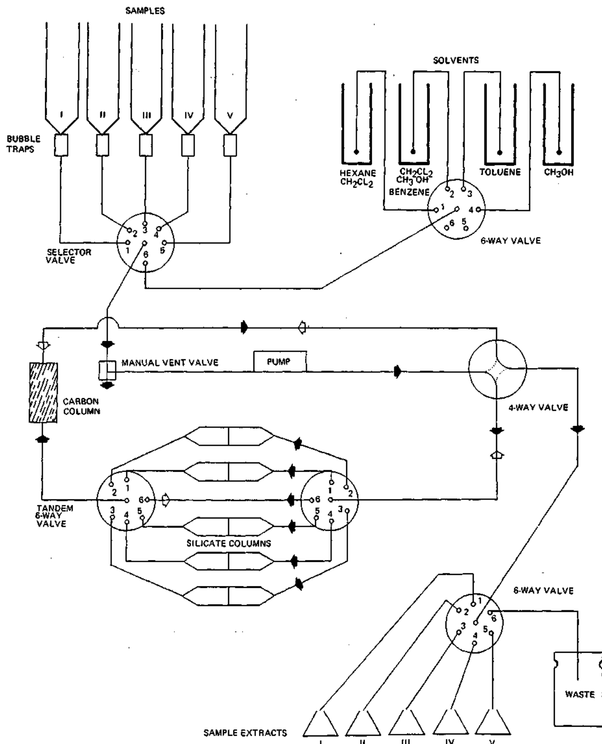
Figure 1. Apparatus used to automate extraction and cleanup part of method for the analysis of tissue samples for 2,3,7,8-tetrachloro-dibenzo- p -dioxin.
